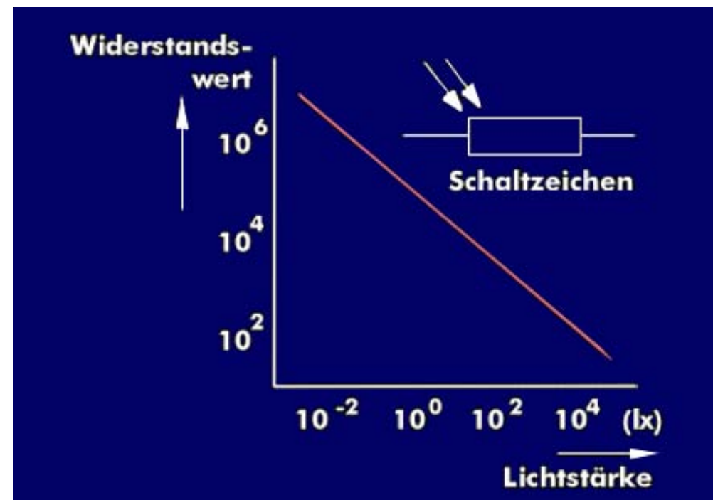
Fotowiderstand LDR, light dependent resistor
